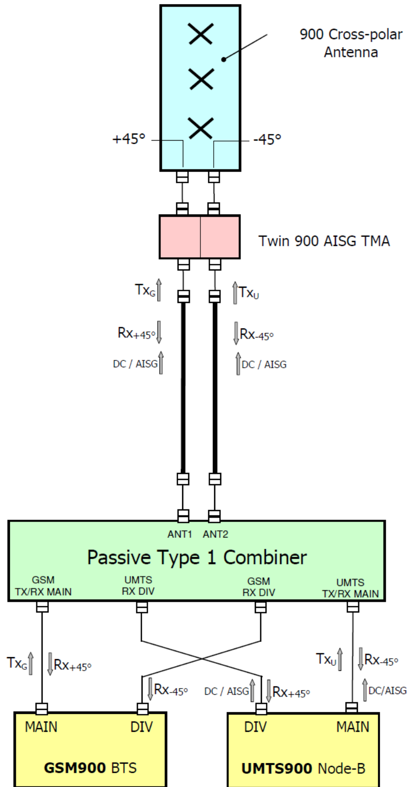
Figure 5 Passive Type 1 Combiner - System Block Diagram
