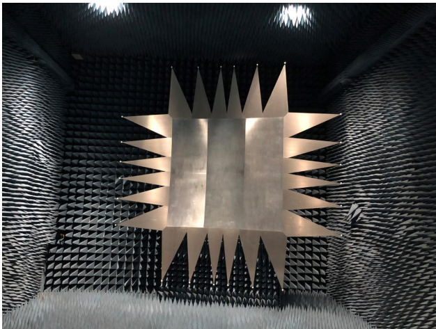
The serrated edge parabolic reflector.
