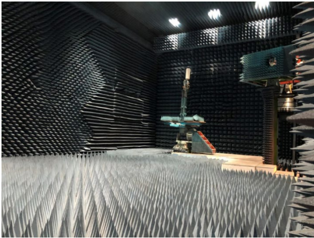
The compact, far-field anechoic chamber located at the Design Center in Täby, Sweden
