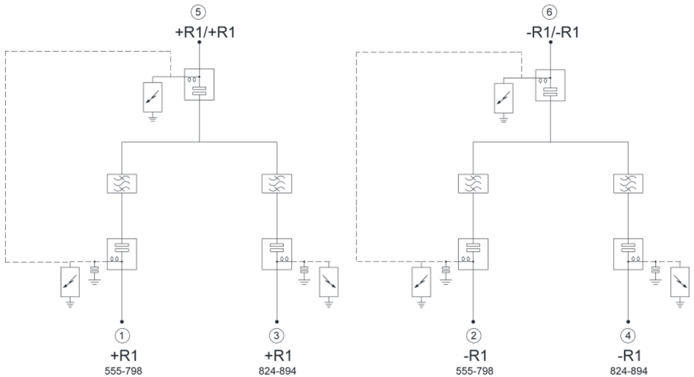
TWIN ELECTRICAL DIAGRAM
