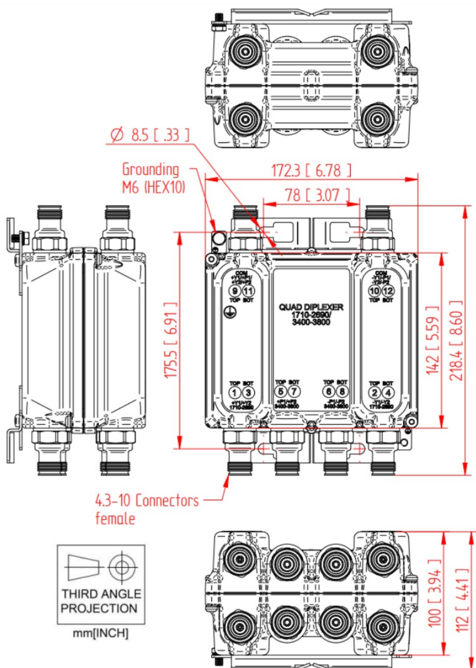
DBCT155F1VXX-1 SINGLE MOUNT
