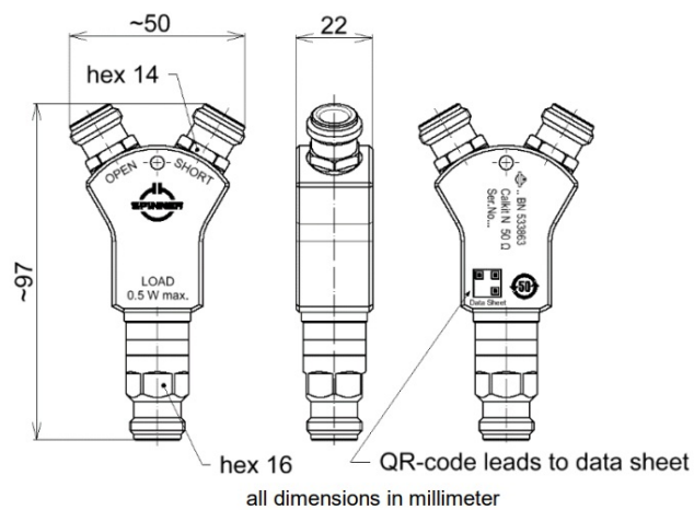
R29-4455 - OSL Compact Calibration Kit - N type Female connectors
