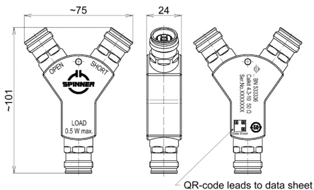
CA123899 - OSL Compact Calibration Kit - 4.3-10 Female connectors
