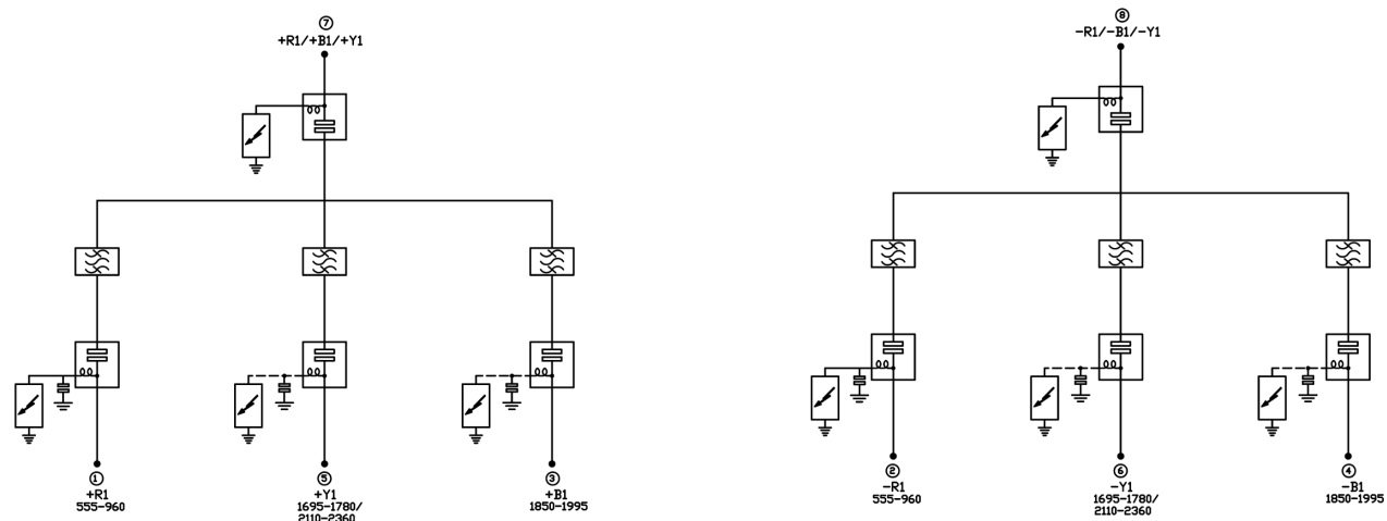
SINGLE TWIN SCHEMATIC
